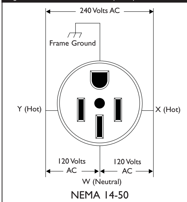
Figure 15 — 120/240 Volt AC, 50 Amp Receptacle
